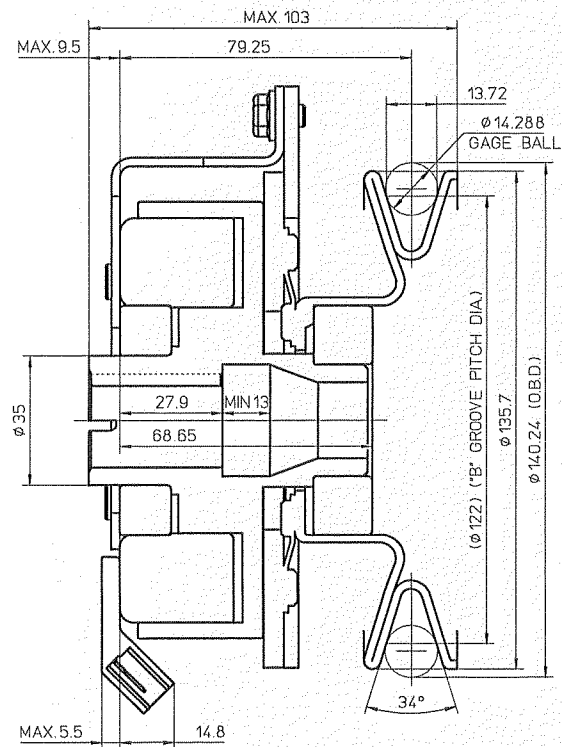
SECTION Z-Z
