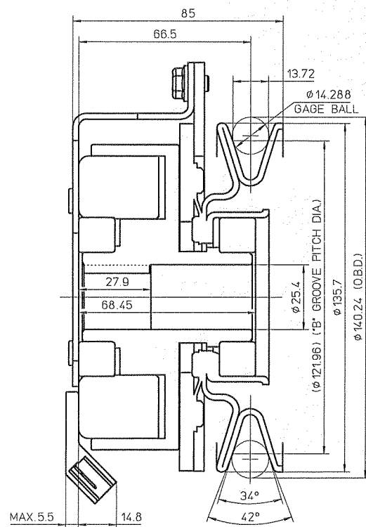
SECTION Z-Z
