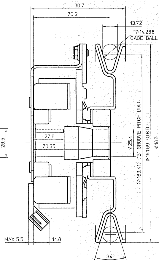
SECTION Z-Z
